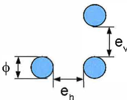
Figure 8.201 — Clear distances between reinforcement
