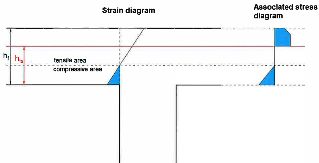
Figure 6.203 — Diagram of the web/flange joint
