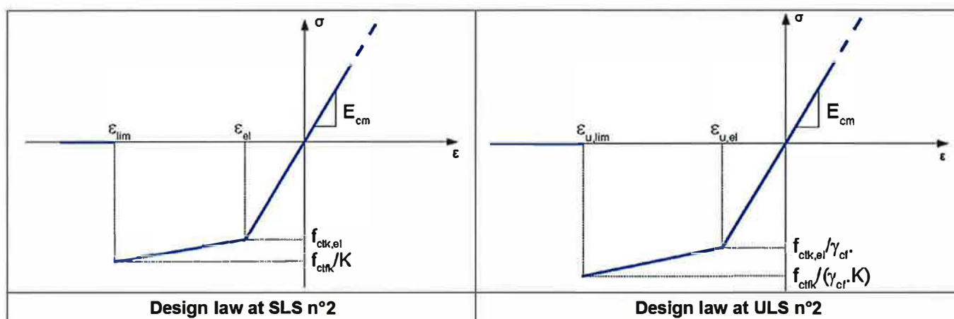
Figure 3.208 — Conventional law n°. 2 for thin members
