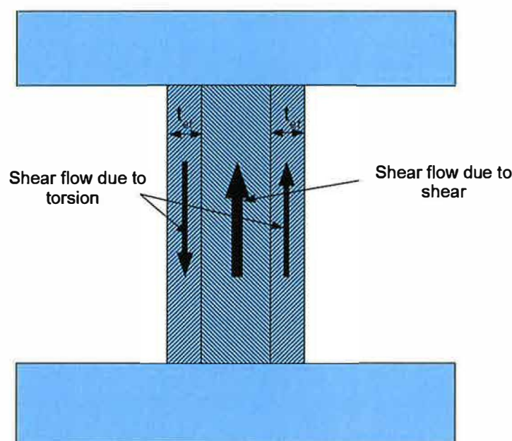
Figure 6.207 — Shear flow due to torsion and shear
