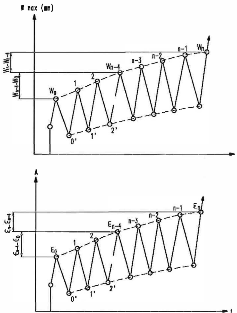
Figure S.3 — Assessment of stabilisation of strain and crack widths
