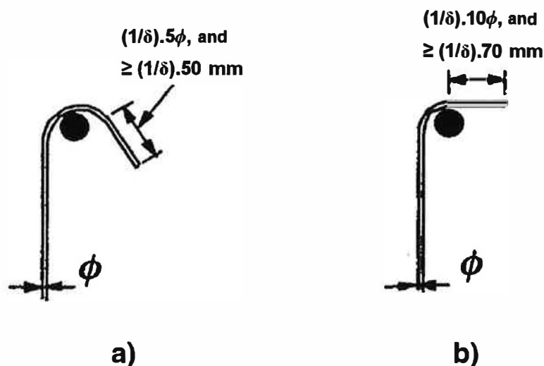
Figure 8.202 — Anchorage of links
