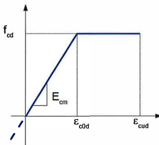
Figure 3.202 — Representation of the stress-strain relation of UHPFRC in compression for designs at ULS
