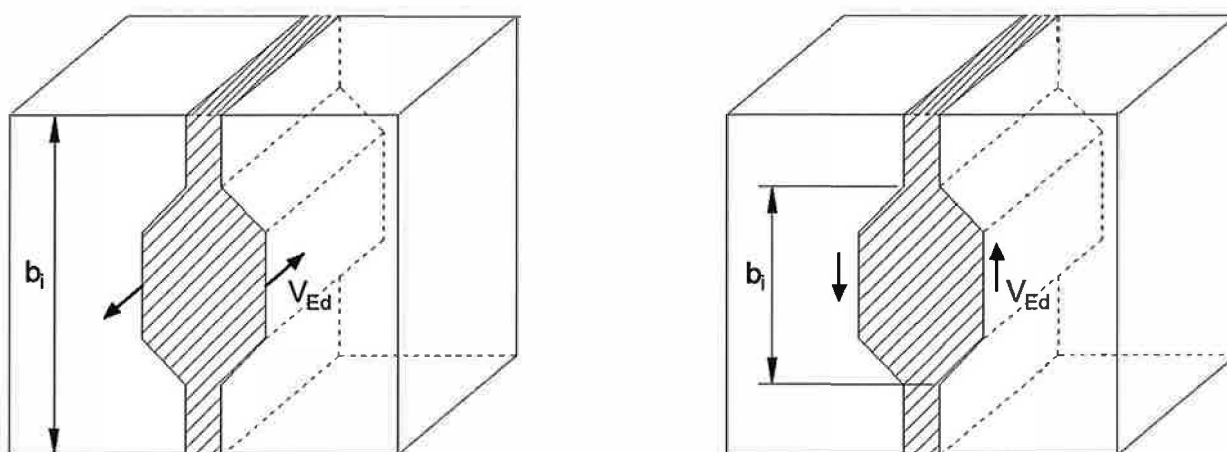
Figure 6.205 — Example de concreting joint areas
