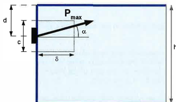
Figure J.103 — Primary regularisation prism – longitudinal view
