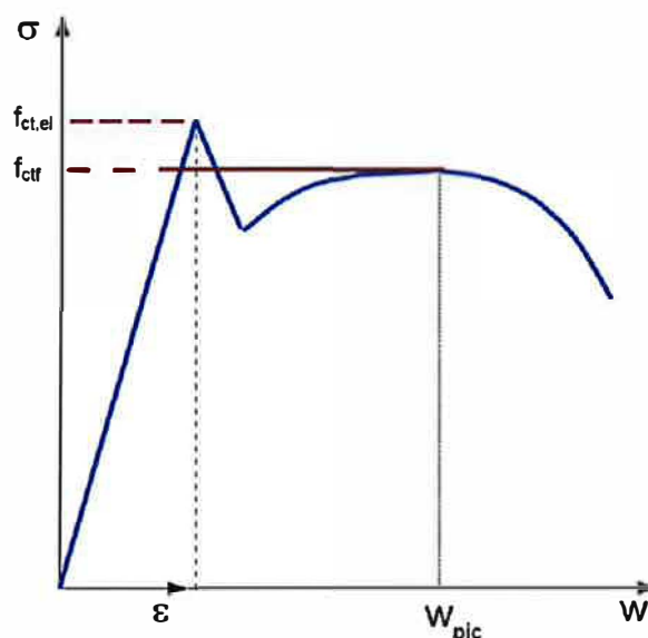
Figure 3.203 — Definition of f_{ctf} in the case of a local maximum
