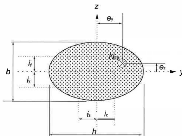
Figure 5.8 — Definition of eccentricities e_y and e_z
