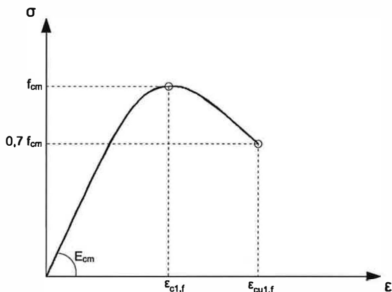
Figure 3.201 — Representation of the stress-strain relation of UHPFRC in compression for non-linear structural analysis
