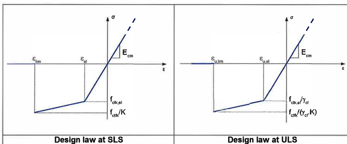
Figure 3.206 — Law for UHPFRCs of class T3* (obtained directly in \sigma(\varepsilon) )
