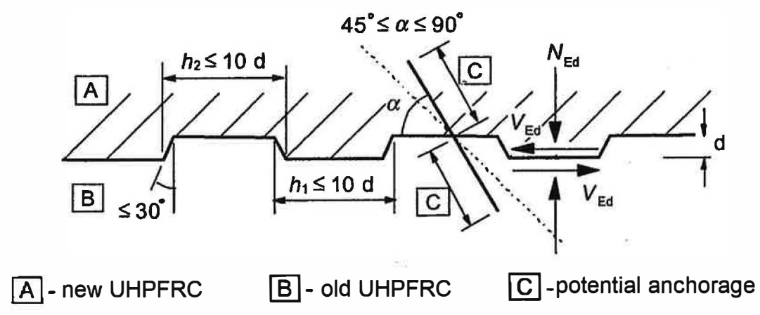
Figure 6.206 — Indented construction joint
