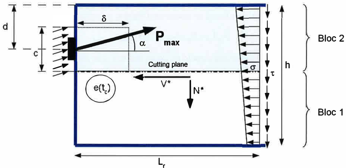
Figure J.105 — Calculation of forces at the cutting planes
