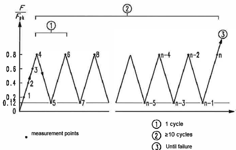
Figure S.2 — Load transfer test procedure
