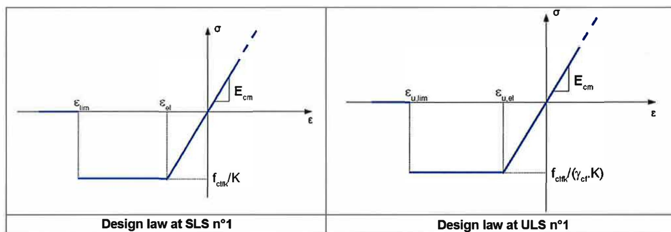
Figure 3.207 — Conventional law n°. 1 for thin members
