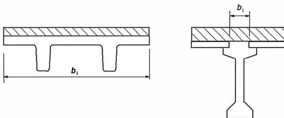
Figure 6.204 — Examples of joint area in composite section
