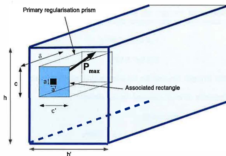
Figure J.102 — Primary regularisation prism
