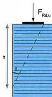
Figure J.101 — Edge sliding mechanism
