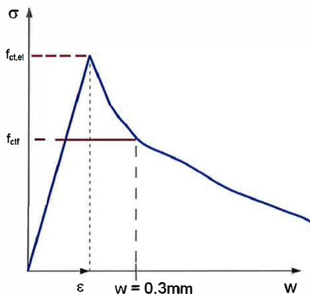
Figure 3.204 — Definition of f_{ctf} in the case where there is no local maximum
